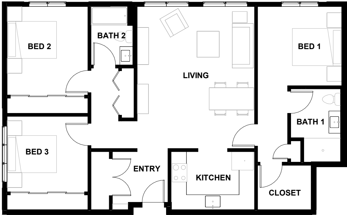
1 3-BEDROOM UNIT PLAN 1,200 FT 2 1/8" = 1'-0"
